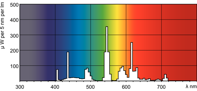
LDPO_TL5-HO8_835-Spectral power distribution Colour
